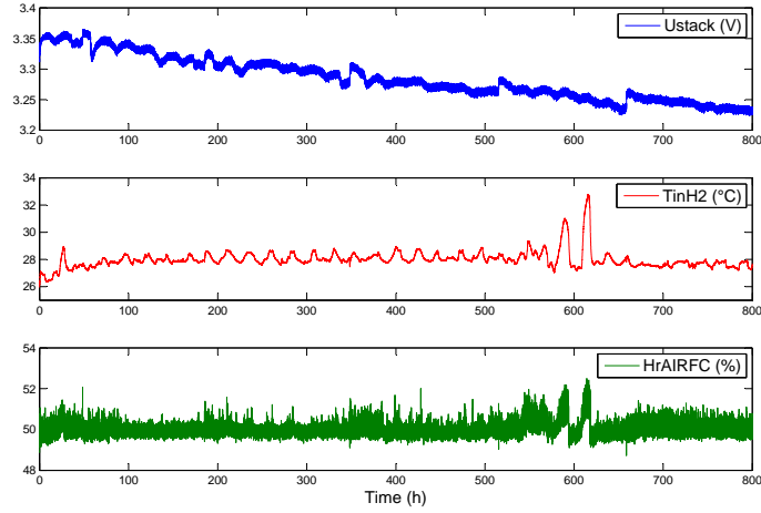
Figure 3: FC1 - example of monitoring index
